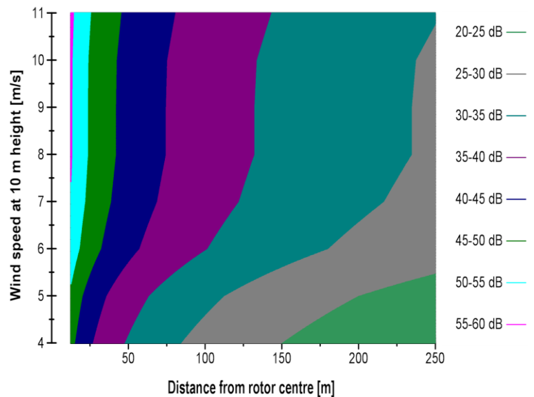
Acoustic Noise Level
