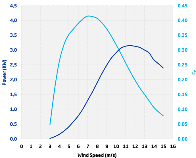
Power and C_p Curve
